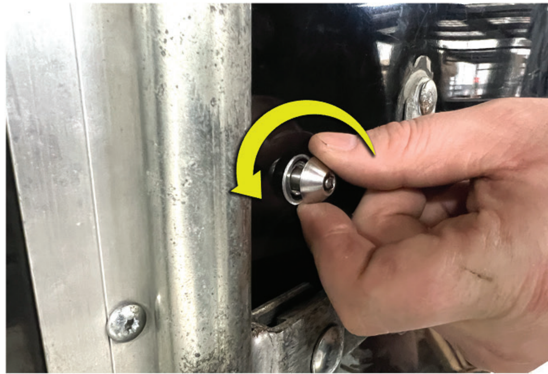
Turn the pin by hand and make sure it is threading into the anchor without cross threading. It may be necessary to realign the Lock Pin into the Anchor.
