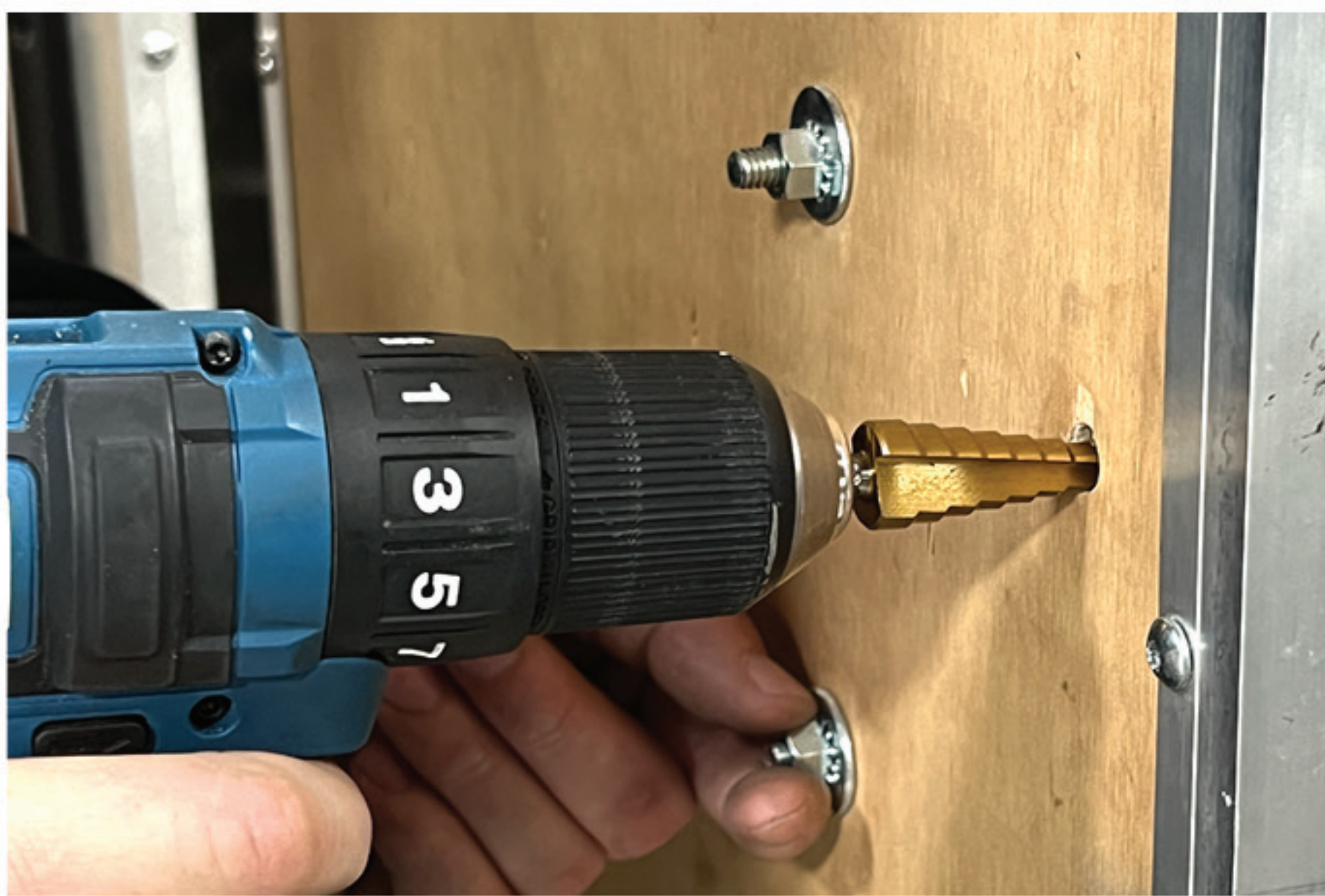
Do the same on the inside of the door using the step bit.
