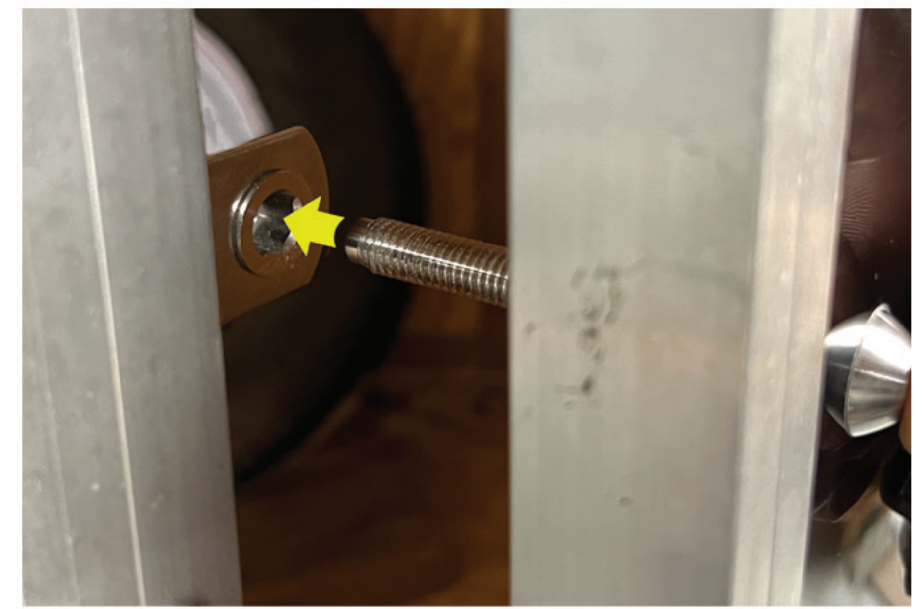
Be sure the Lock Pin aligns with the Anchor when shutting/securing the door.
